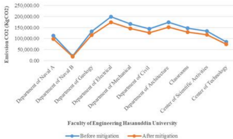
Figure 5. CO 2 emission before and after 1 hour shutdown
